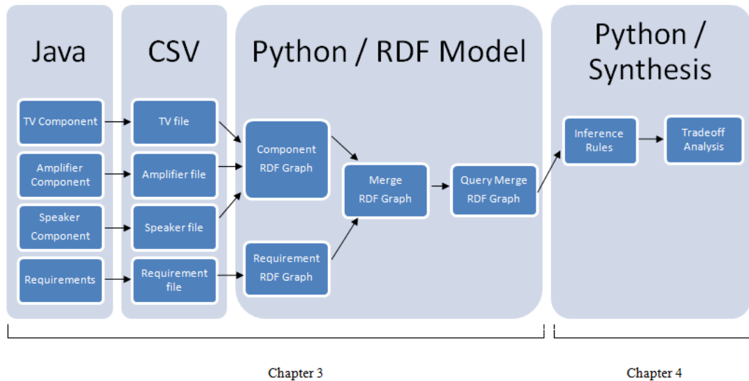
Figure 1.14: Flowchart for systems modeling with Java and Python.
